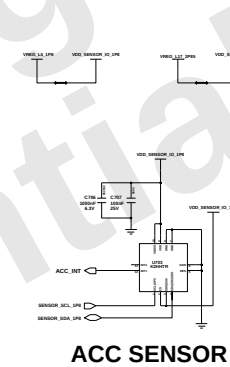
ACC SENSOR
