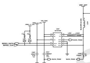
APT MODULATOR
