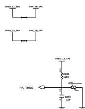
THERMISTER
